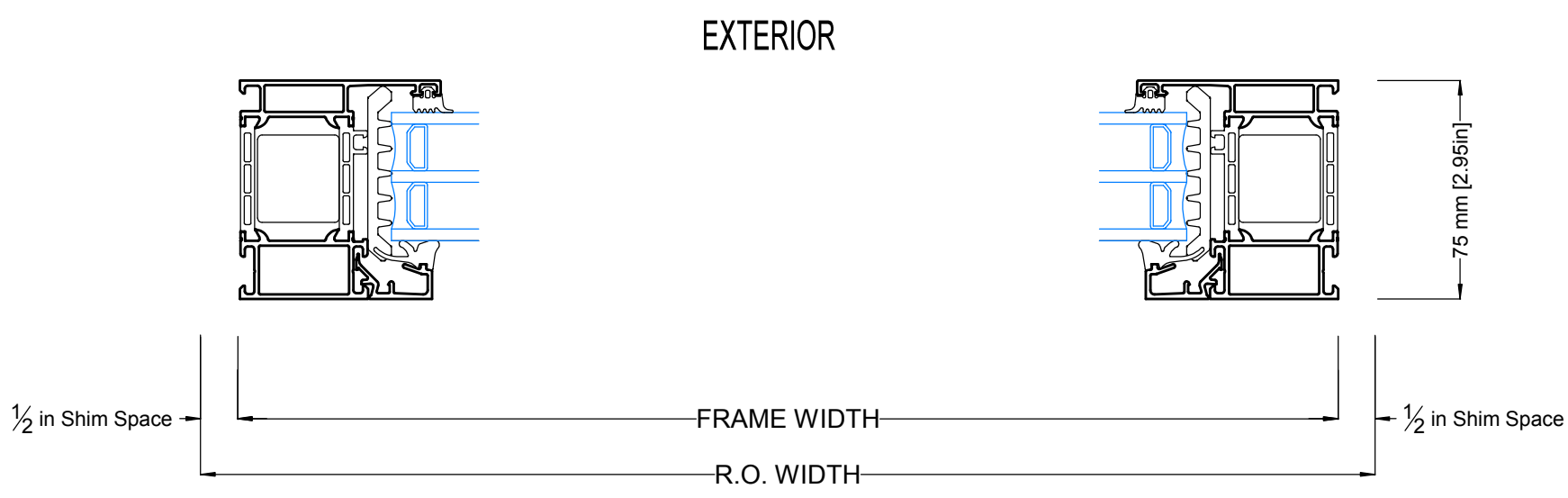
JAMB DETAIL FIXED WINDOWS
